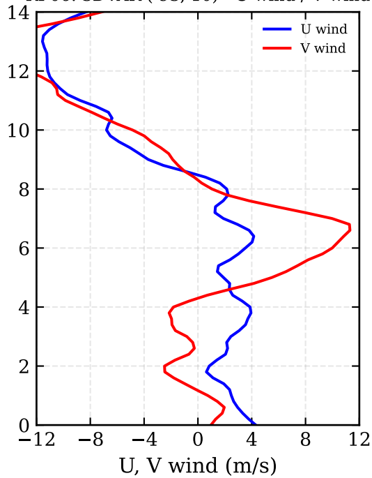
RF06: 3DVAR (-93, 10) - U wind / V wind
