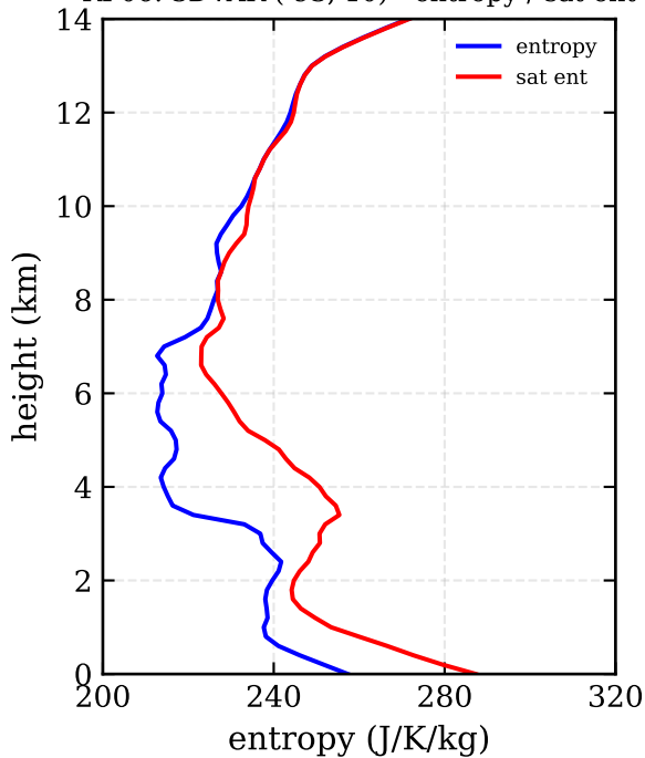
RF06: 3DVAR (-93, 10) - entropy / sat ent
