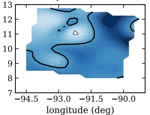
RF06, day 230, srcent ( \text{W/m}^2 )
