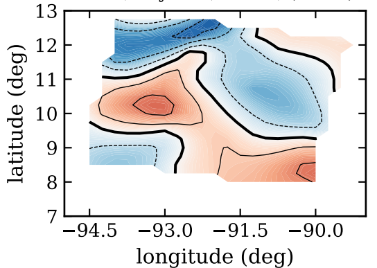
RF06, day 230, srcmr, ( \text{W/m}^2 )
