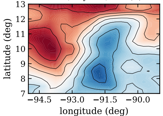
RF06, day 230, SST (C)
