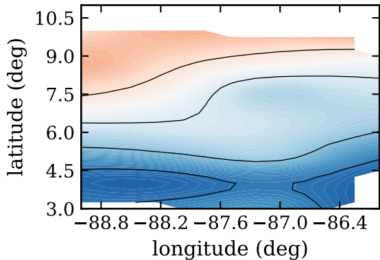
RF08, day 235, instab index (J/K/kg)
