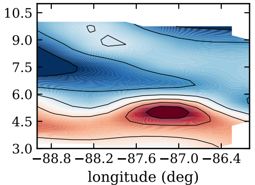
RF08, day 235, satfrac
