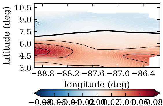
RF08, day 235, mfluxvl (kg/m 2 /s)
