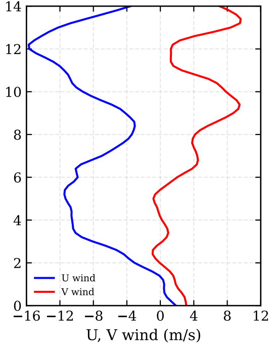
RF08: 3DVAR (-89.0, 5.0) - U wind / V wind
