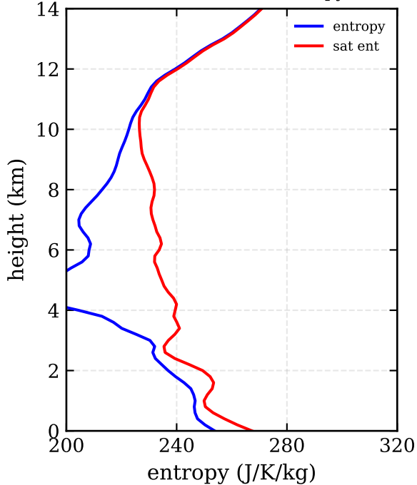
RF08: 3DVAR (-89.0, 5.0) - entropy / sat ent
