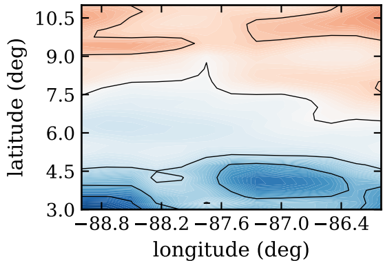
RF08, day 235, SST (C)
