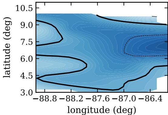
RF08, day 235, dcin, (J/K/kg)
