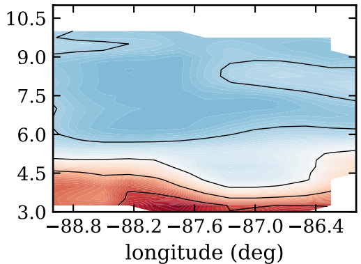
RF08, day 235, eflux (W/m 2 )
