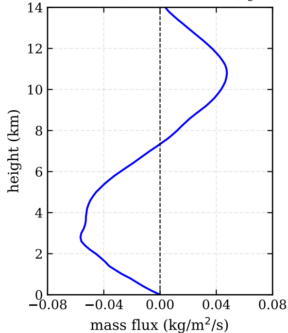
RF09a: 3DVAR (-79, 7) - mass flux ( \text{kg}/\text{m}^2/\text{s} )
