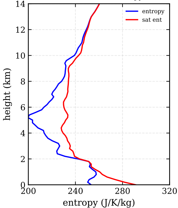
RF10: 3DVAR (-82, 10) - entropy / sat ent
