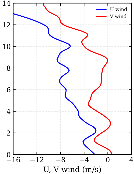
RF10: 3DVAR (-82, 10) - U wind / V wind
