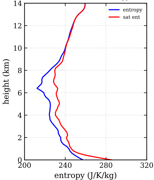
RF13c: 3DVAR (-79.5, 5.8) - entropy / sat ent
