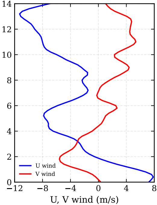
RF13c: 3DVAR (-79.5, 5.8) - U wind / V wind
