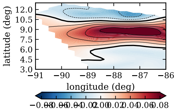
RF14, day 264, mfluxvl (kg/m 2 /s)
