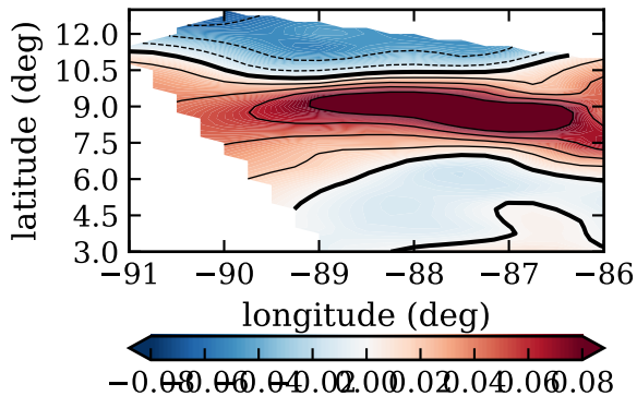
RF14, day 264, mfluxlo (kg/m 2 /s)
