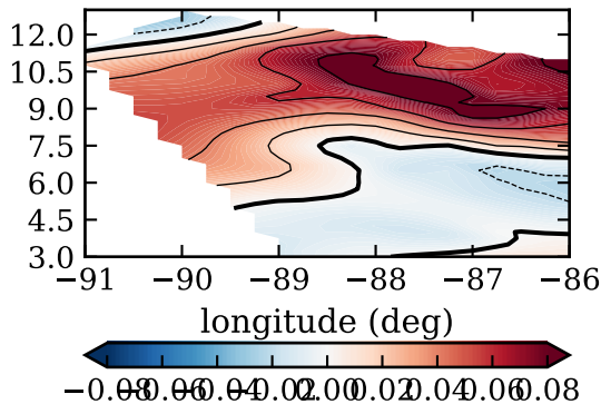
RF14, day 264, mfluxhi (kg/m 2 /s)
