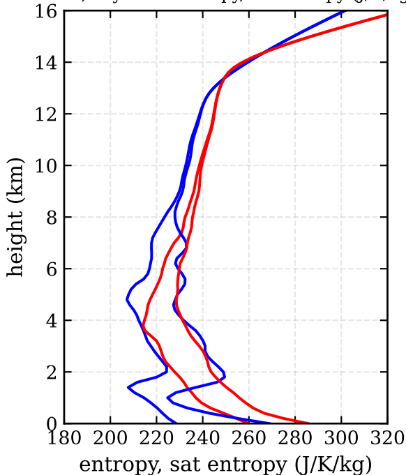
RF14, day 264 - entropy, sat entropy (J/K/kg)
