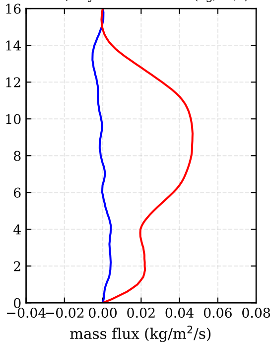
RF14, day 264 - mass flux (kg/m 2 /s)
