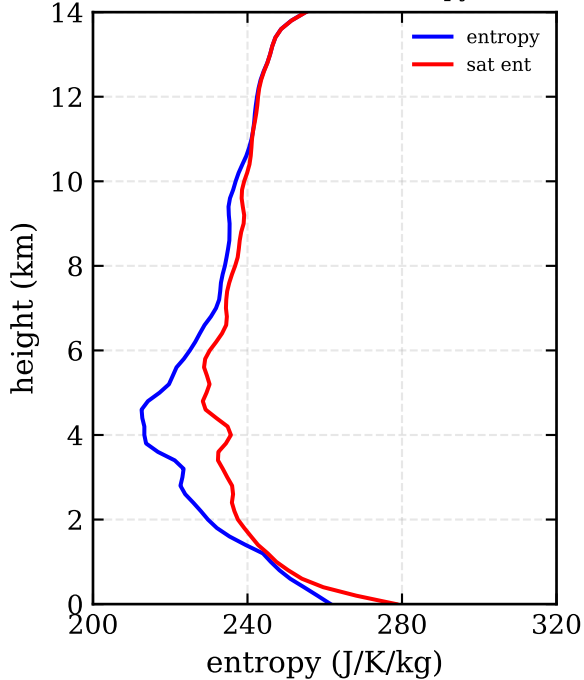
RF14: 3DVAR (-87, 8.5) - entropy / sat ent
