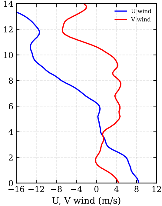
RF14: 3DVAR (-87, 8.5) - U wind / V wind
