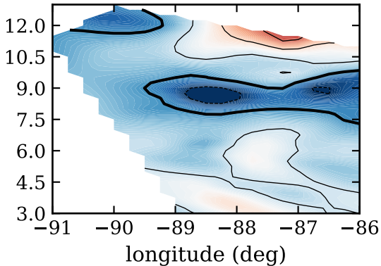
RF14, day 264, srcent ( \text{W/m}^2 )
