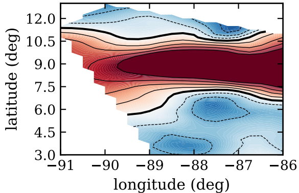
RF14, day 264, srcmr, ( \text{W/m}^2 )
