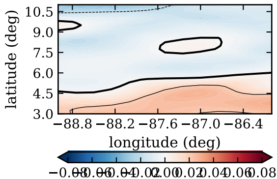
RF16, day 267, mfluxvl (kg/m 2 /s)
