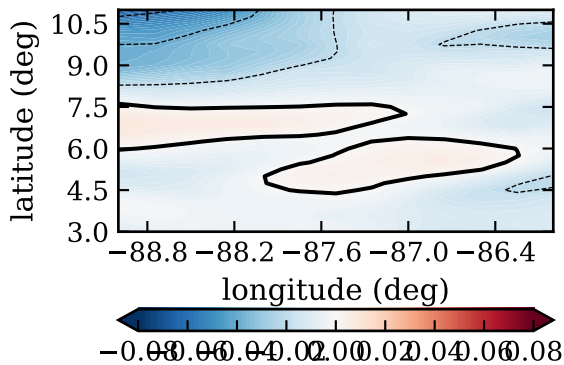
RF16, day 267, mfluxlo (kg/m 2 /s)
