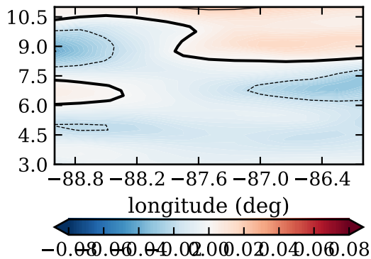
RF16, day 267, mfluxhi (kg/m 2 /s)
