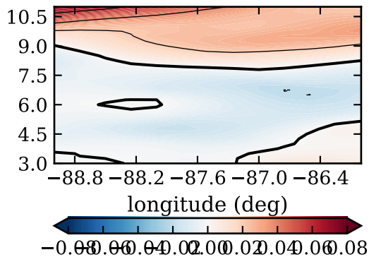
RF16, day 267, mfluxdif (kg/m 2 /s)
