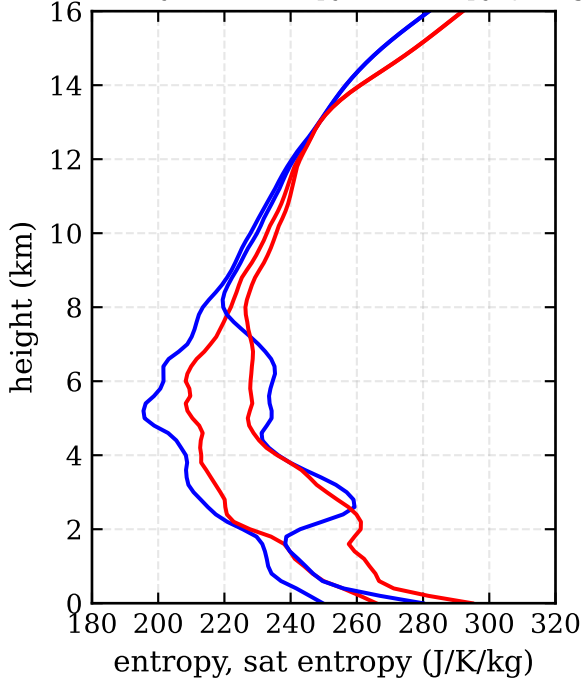
RF16, day 267 - entropy, sat entropy (J/K/kg)
