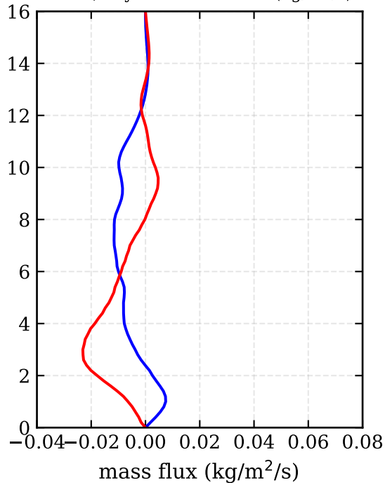
RF16, day 267 - mass flux (kg/m 2 /s)
