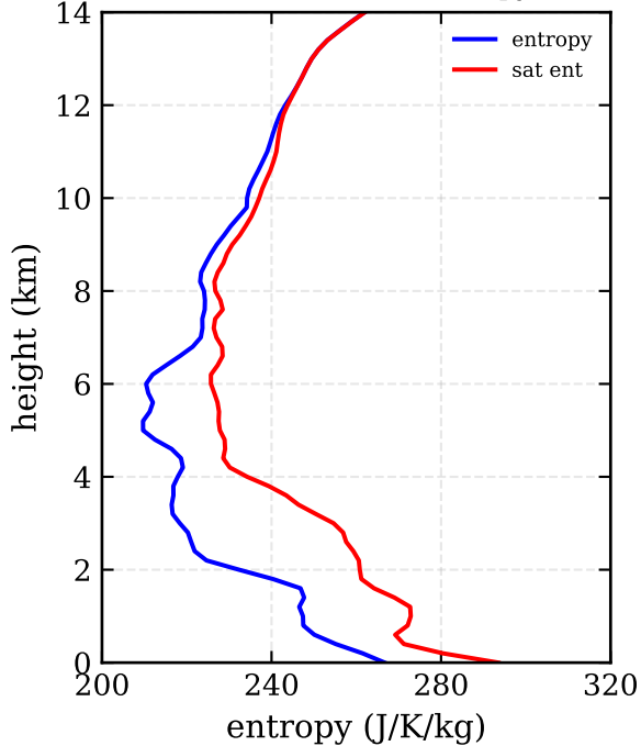
RF16: 3DVAR (-87.5, 9.5) - entropy / sat ent
