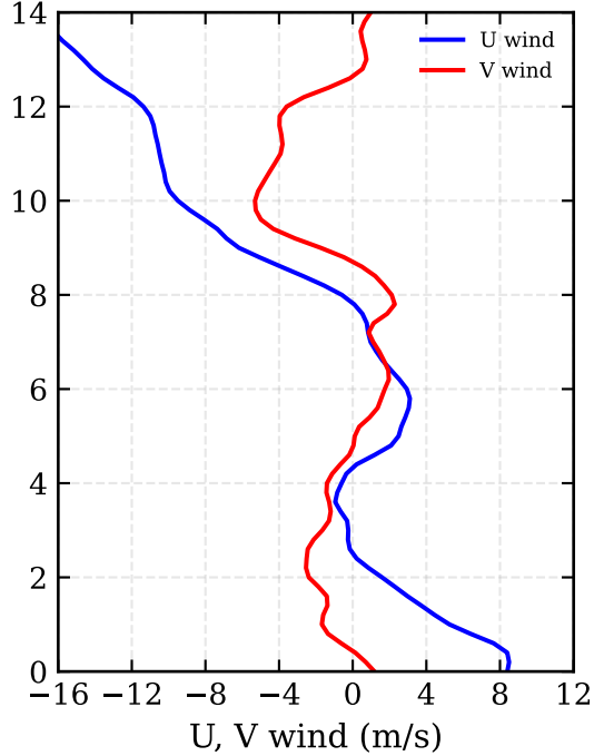
RF16: 3DVAR (-87.5, 9.5) - U wind / V wind
