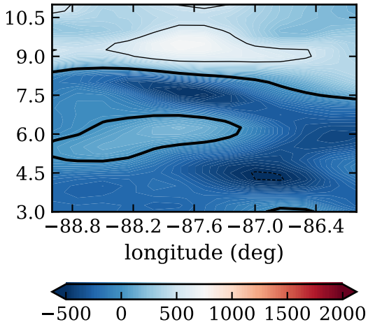
RF16, day 267, srcent ( \text{W/m}^2 )
