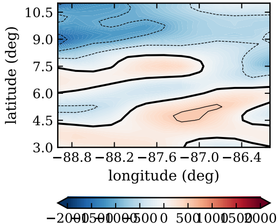
RF16, day 267, srcmr, ( \text{W/m}^2 )
