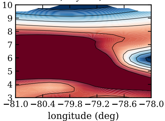
RF17c, day 268, satfrac
