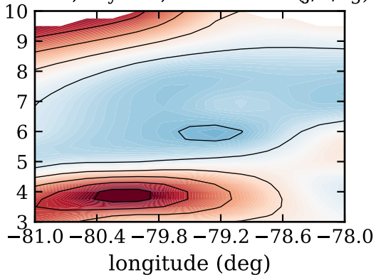
RF17c, day 268, instab index (J/K/kg)
