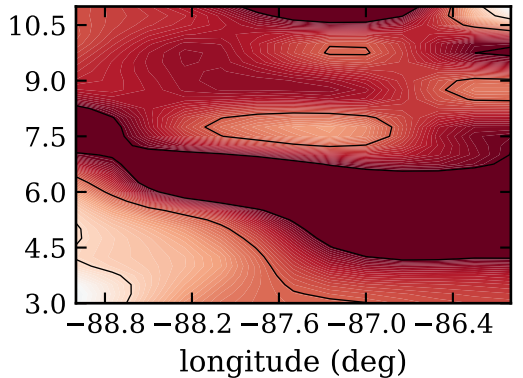
RF18, day 270, satfrac
