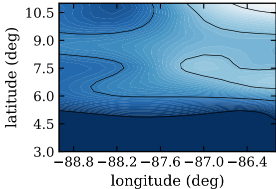
RF18, day 270, instab index (J/K/kg)
