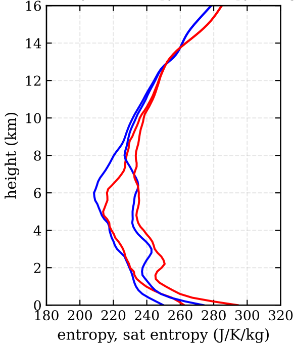
RF18, day 270 - entropy, sat entropy (J/K/kg)
