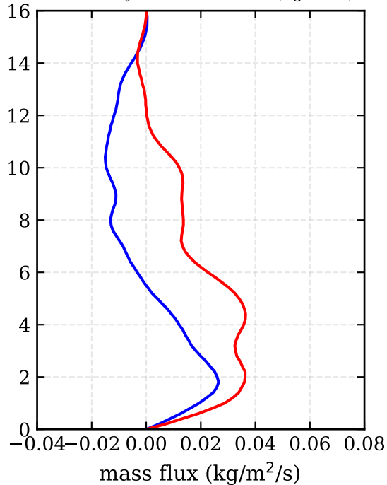
RF18, day 270 - mass flux (kg/m 2 /s)
