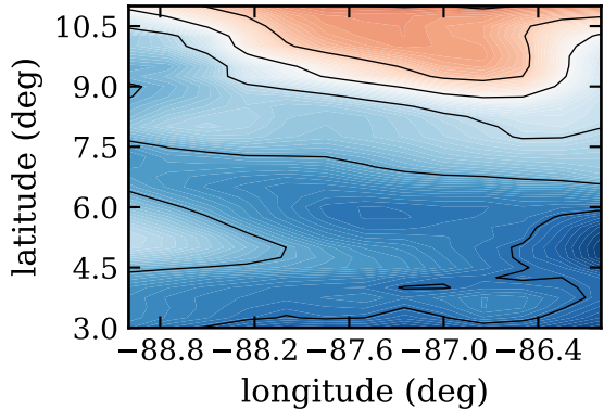
RF18, day 270, SST (C)
