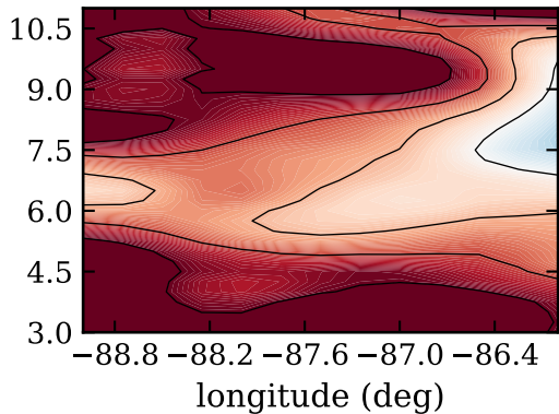
RF18, day 270, eflux (W/m 2 )
