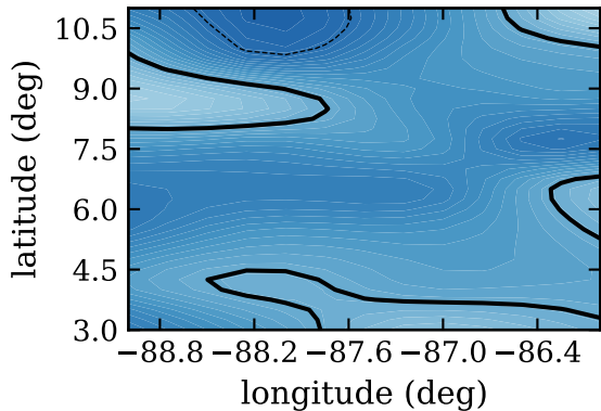
RF18, day 270, dcin, (J/K/kg)
