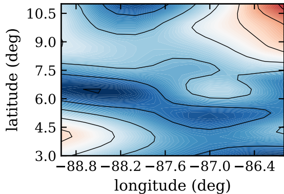
RF19, day 271, instab index (J/K/kg)
