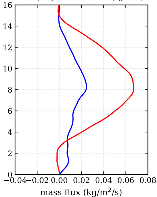
RF19, day 271 - mass flux (kg/m 2 /s)
