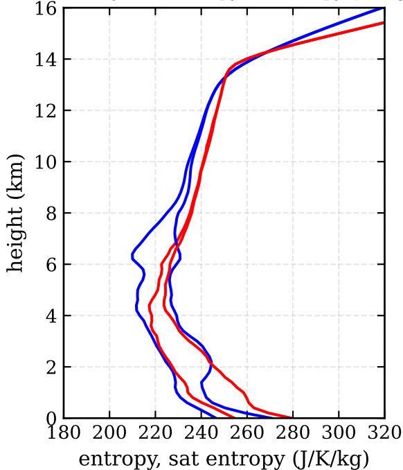
RF19, day 271 - entropy, sat entropy (J/K/kg)
