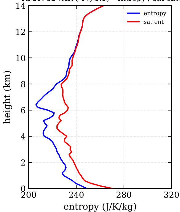
RF19: 3DVAR (-87, 5.5) - entropy / sat ent
