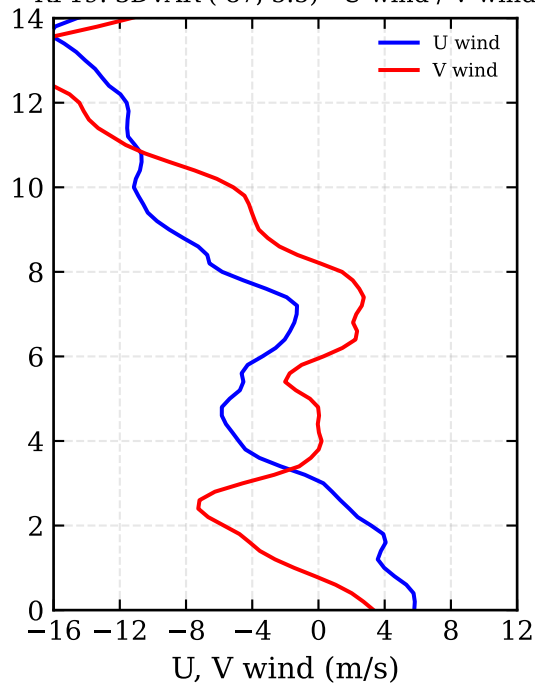
RF19: 3DVAR (-87, 5.5) - U wind / V wind
