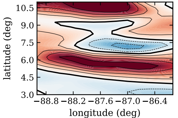
RF19, day 271, srcmr, ( \text{W}/\text{m}^2 )
