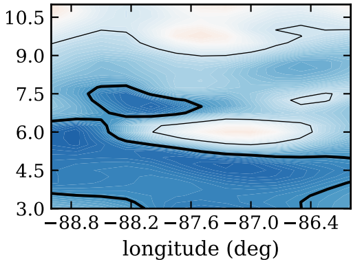
RF19, day 271, srcent ( \text{W}/\text{m}^2 )
