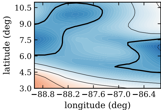
RF19, day 271, dcin, (J/K/kg)
