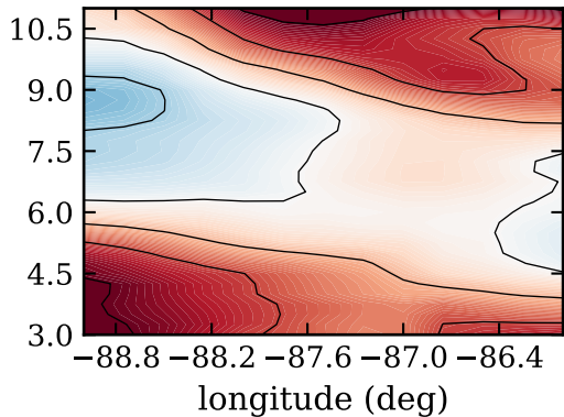
RF19, day 271, eflux (W/m 2 )
