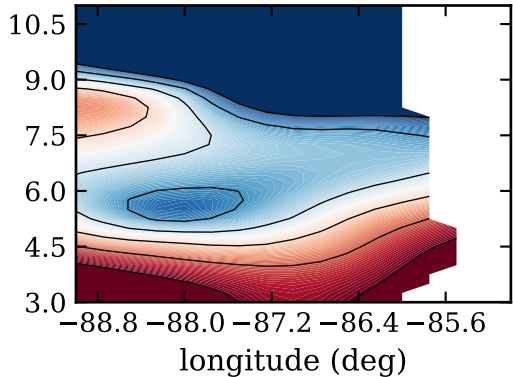
RF20, day 273, satfrac
