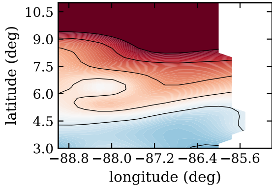
RF20, day 273, instab index (J/K/kg)
