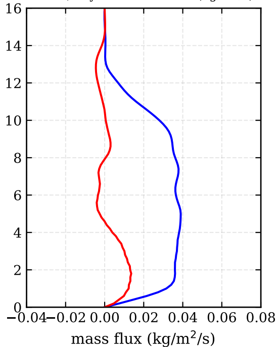
RF20, day 273 - mass flux (kg/m 2 /s)
