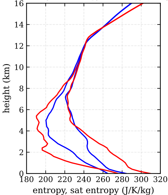
RF20, day 273 - entropy, sat entropy (J/K/kg)
