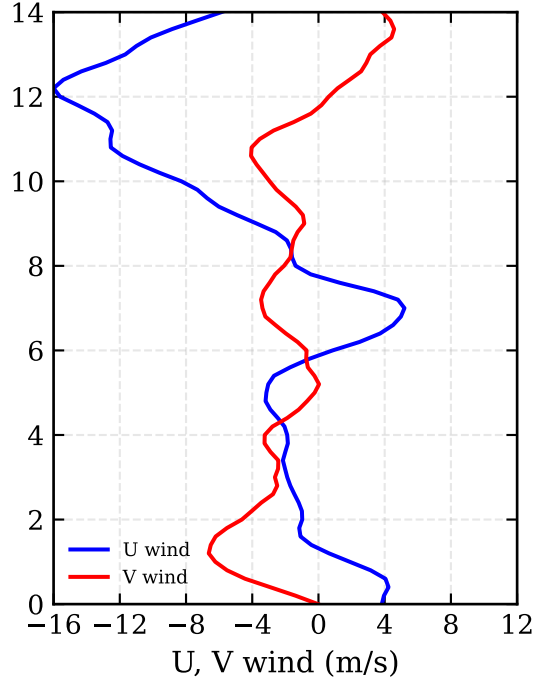
RF20: 3DVAR (-89, 4.5) - U wind / V wind
