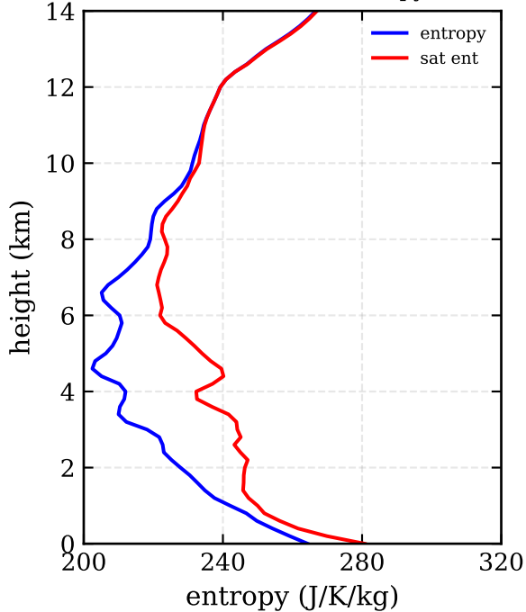
RF20: 3DVAR (-89, 4.5) - entropy / sat ent
