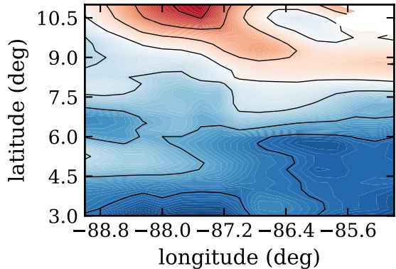
RF20, day 273, SST (C)
