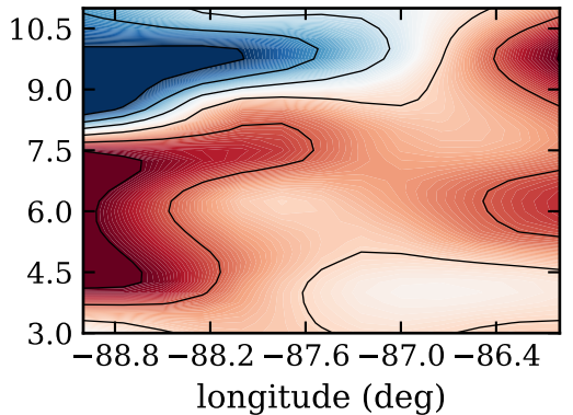
RF21, day 274, satfrac
