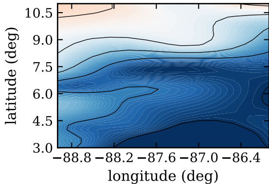
RF21, day 274, instab index (J/K/kg)
