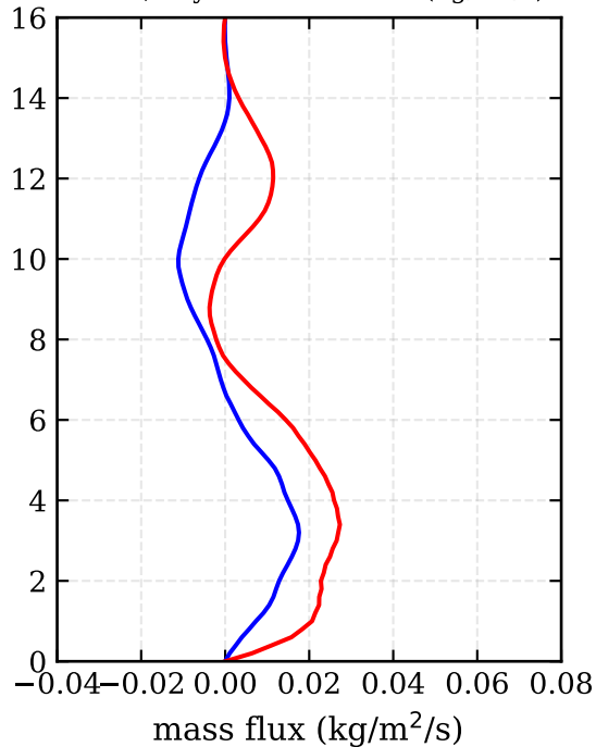
RF21, day 274 - mass flux (kg/m 2 /s)
