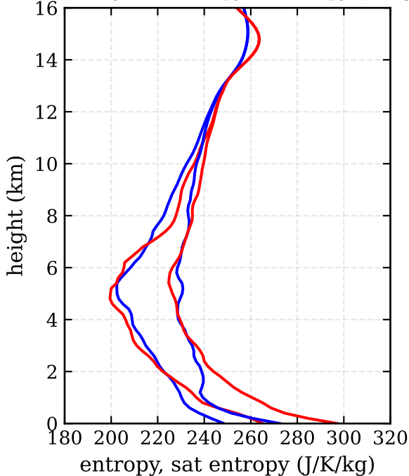
RF21, day 274 - entropy, sat entropy (J/K/kg)
