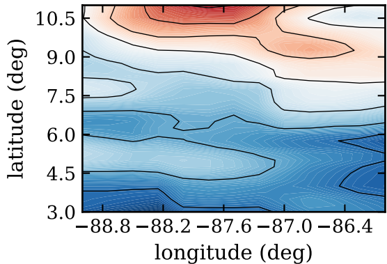
RF21, day 274, SST (C)
