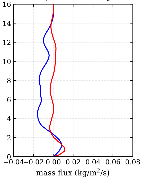
RF22, day 275 - mass flux (kg/m 2 /s)
