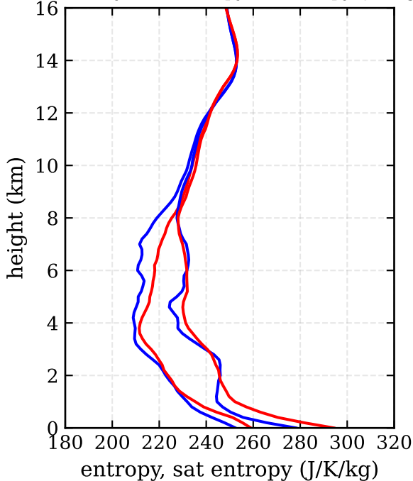
RF22, day 275 - entropy, sat entropy (J/K/kg)
