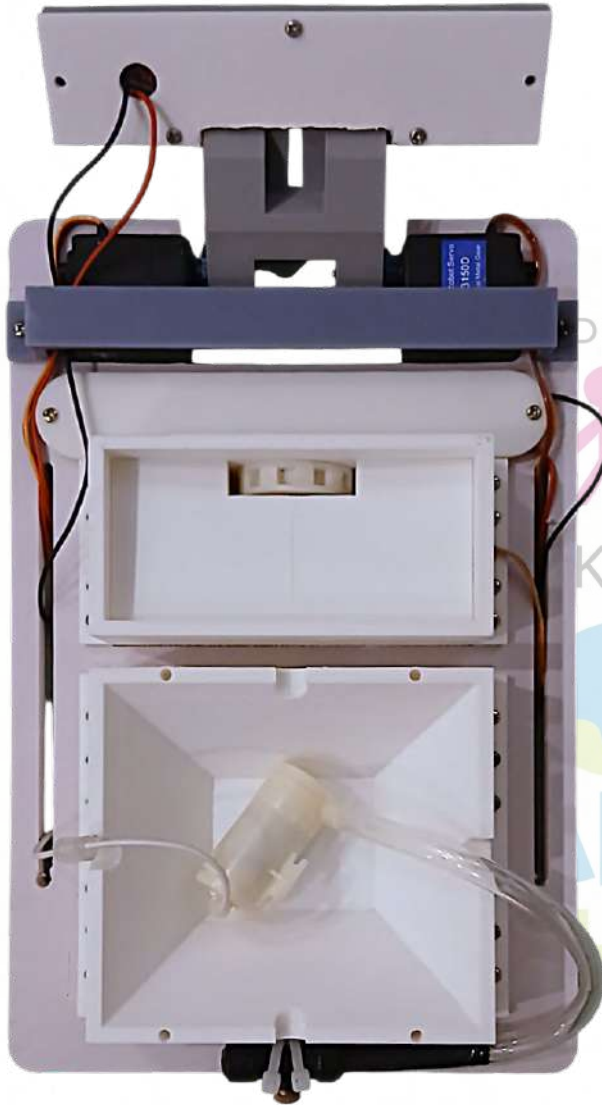
Figure 14: Watering compartment fastened to the baseplate (15cm x 12cm). The container is shaped to funnel water toward the pump intake, which feeds a rear-mounted sprinkler via a connecting pipe. The compartment includes side openings for wire and pipe routing.
