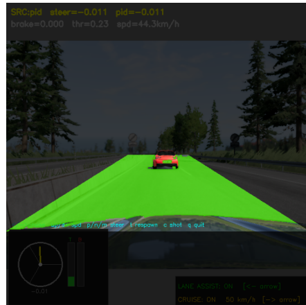
(c) After ROI clipping (green = pixels fed to Hough)
