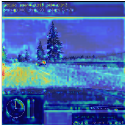
Grad-CAM — steer head \hat{\delta}
