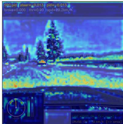
Grad-CAM — brake head \hat{b}
