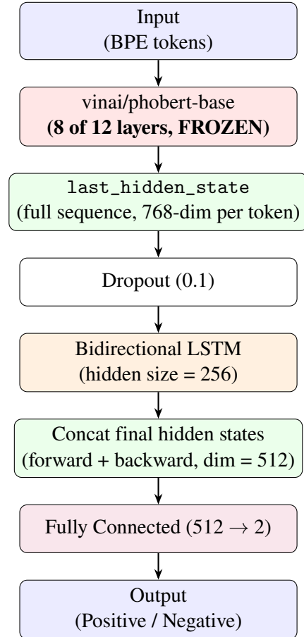
Figure 3.5: Proposed Hybrid PhoBERT-BiLSTM architecture, using a truncated (8-layer), frozen PhoBERT encoder.
