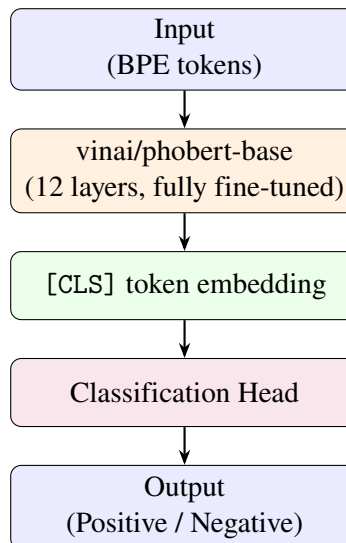
Figure 3.4: PhoBERT model architecture.
