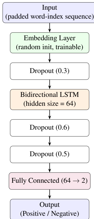
Figure 3.3: BiLSTM model architecture.
