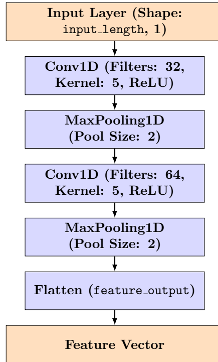
Figure 2: Internal diagram of Temporal Convolution Network used for feature extraction
