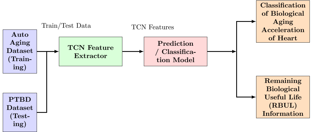
Figure 1: Functional Flow Diagram
