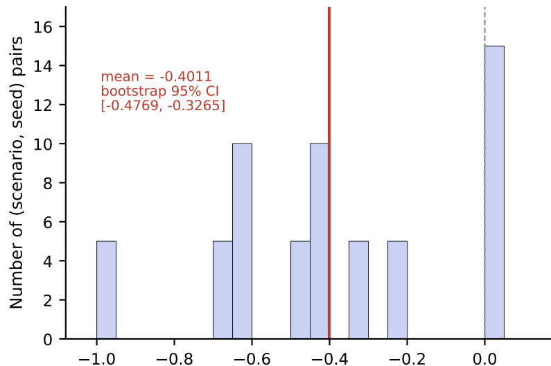
(b) Paired differences, D vs B (0 / 15 / 45 D-better / tie / B-better)
