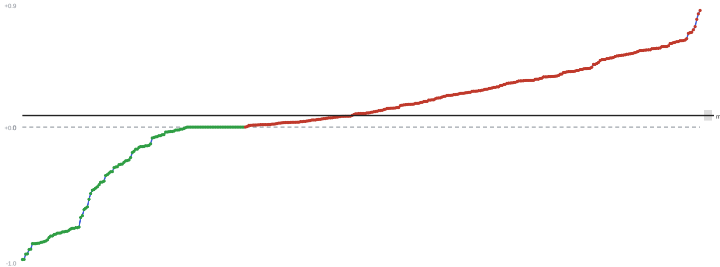
Figure 2 Paired D-B normalised-regret difference, per scenario (sorted) — negative = D better
