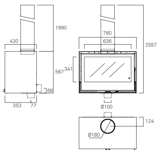
Habit 80 + T + Kit 5★
