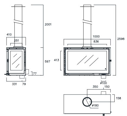
Laria 100 LD + T
