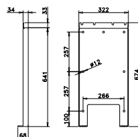
E2100-1 Support mural Habit 50 V + T
