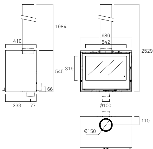
Habit 70 A + T + Kit 5★
