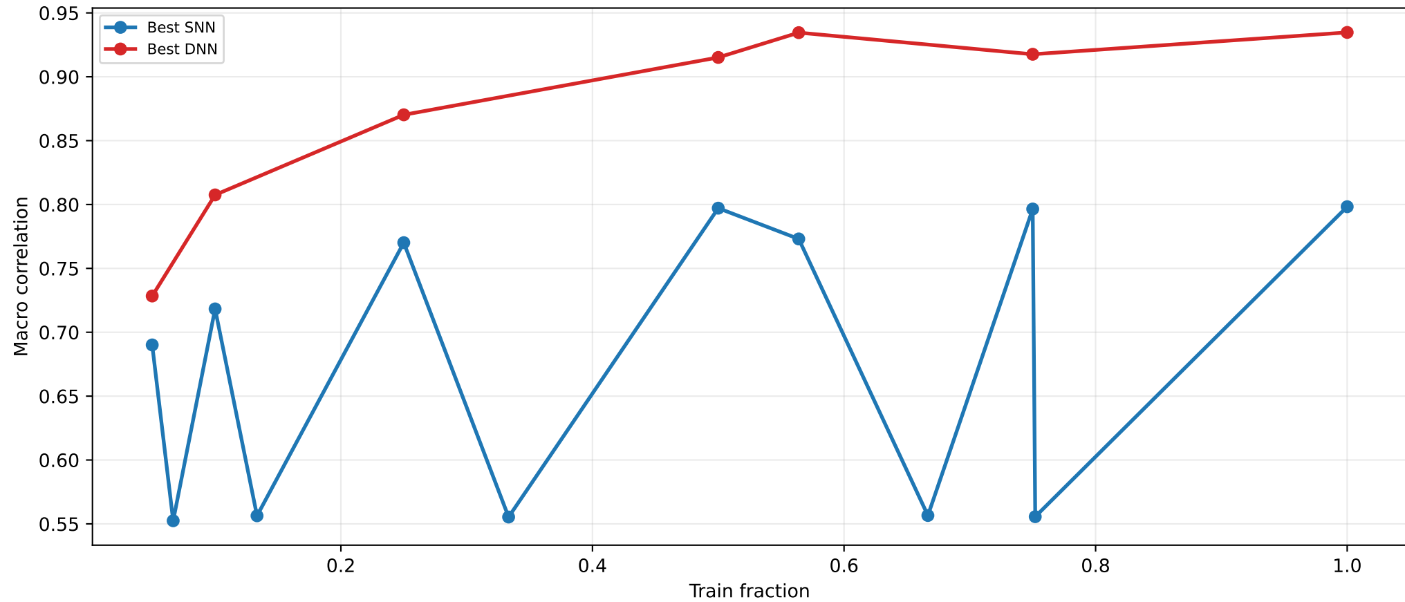
Best SNN vs best DNN macro correlation across train fraction
