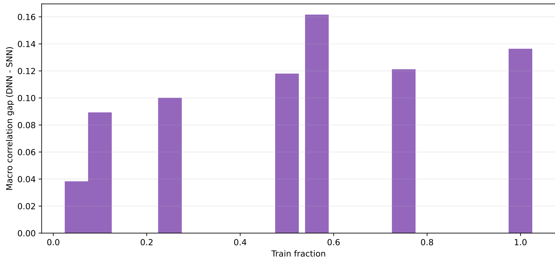
Best DNN minus best SNN macro correlation at each train fraction
