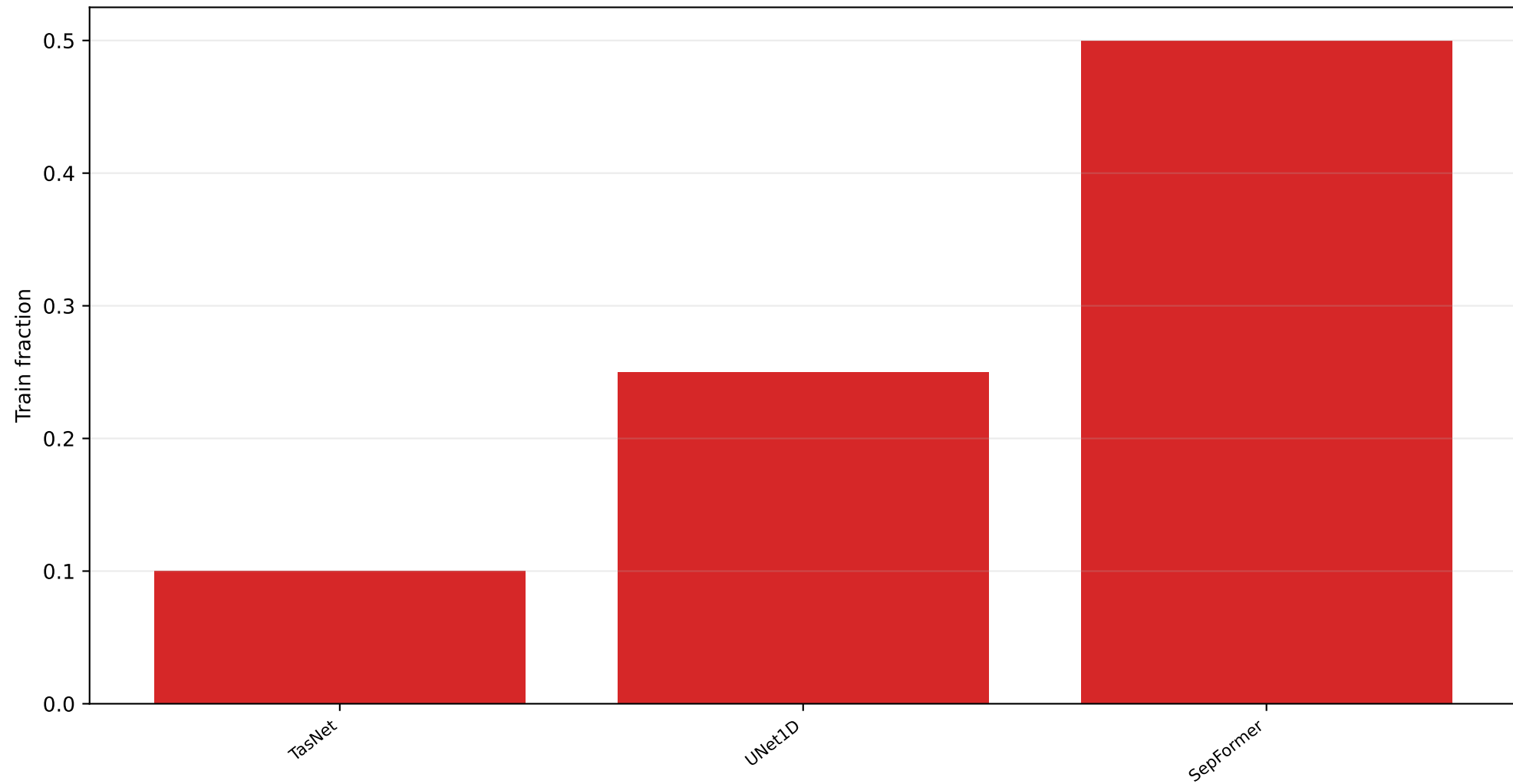
Minimum train fraction to reach macro correlation \geq 0.80
