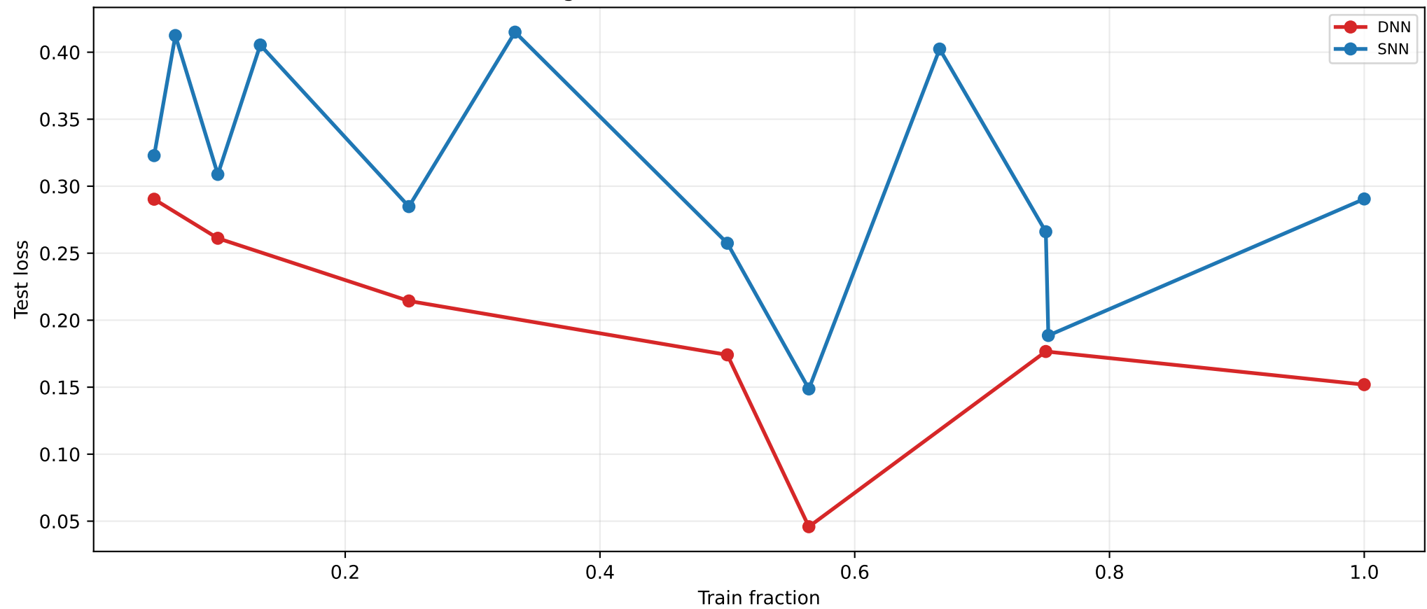
Average SNN vs DNN test loss vs train fraction
