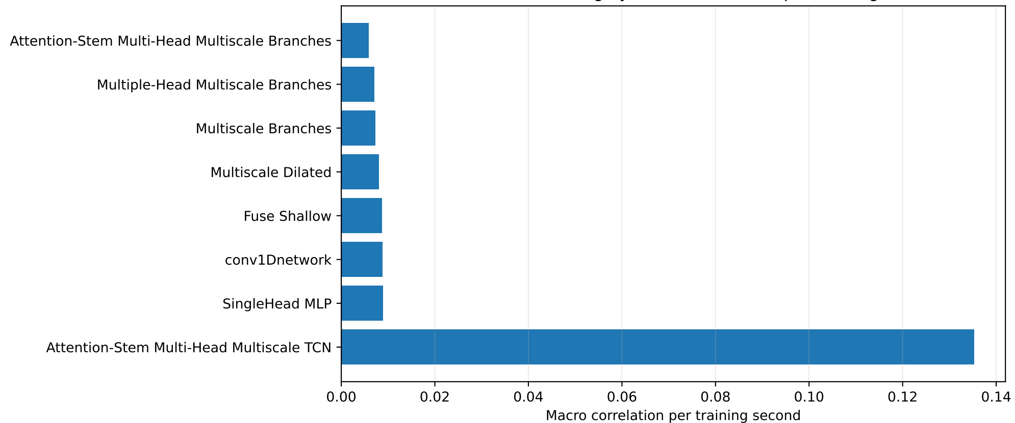
Cost-normalized ranking by macro correlation per training second
